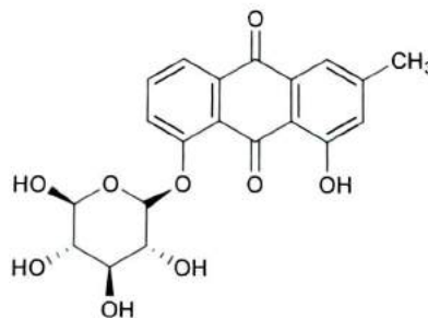
Krisopanol-8-O-glikosida
