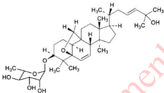
Momordisin
